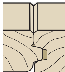
MINI BEVEL \frac{1}{16} "x \frac{1}{16} " bevel ( \frac{1}{8} " overall) V-Groove
