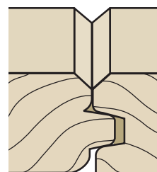
MEDIUM BEVEL \frac{1}{8} "x \frac{1}{8} " bevel ( \frac{1}{4} " overall) V-Groove
