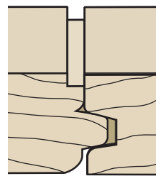
REVEAL EDGE GAP \frac{3}{16} " wide ( \frac{1}{8} " deep)
