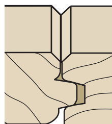
STANDARD BEVEL \frac{3}{32} "x \frac{3}{32} " bevel ( \frac{3}{16} " overall) V-Groove
