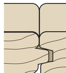
RADIUS EDGE \frac{1}{16} " radius ( \frac{1}{8} " overall)
