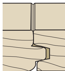
MICRO BEVEL \frac{1}{32} "x \frac{1}{32} " bevel ( \frac{1}{16} " overall) V-Groove
