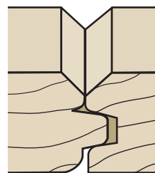
LARGE BEVEL \frac{3}{16} "x \frac{3}{16} " bevel ( \frac{3}{8} " overall) V-Groove
