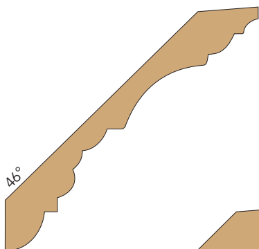
3359 \frac{7}{8} \times 6\frac{5}{8}
